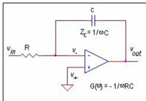
gambar 3 : integrator
