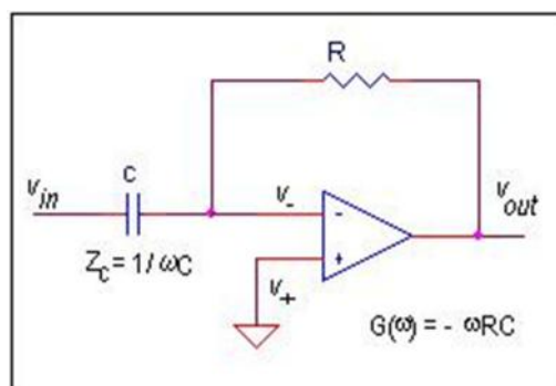
gambar 4 : differensiator
